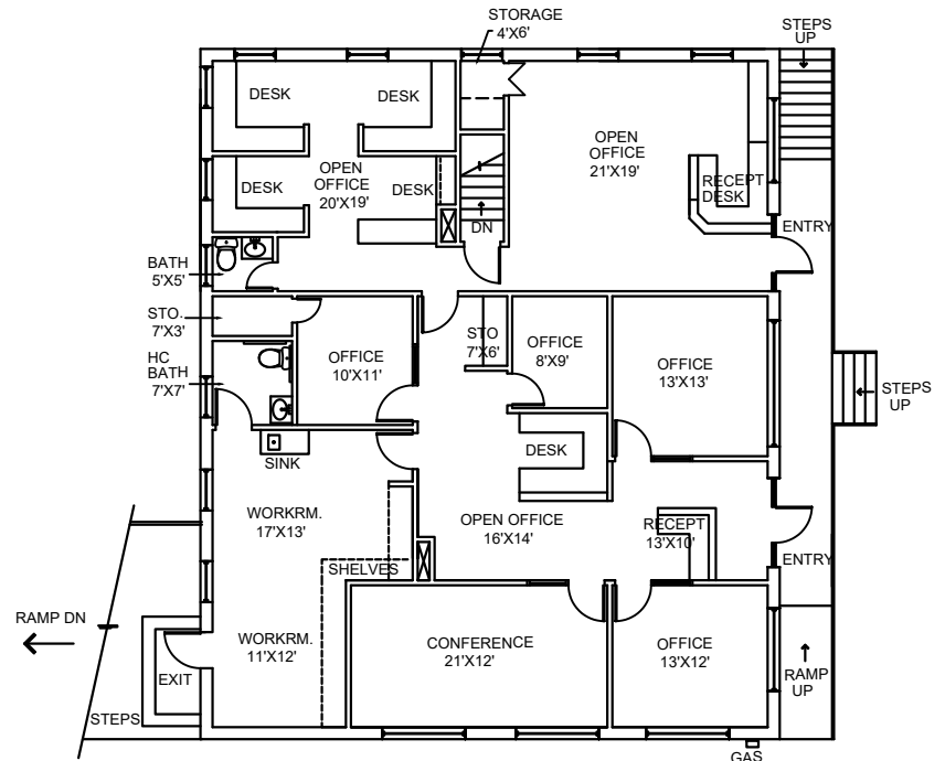
1203 FAY ST. FIRST FLOOR PLAN SCALE: 3/16"=1'-0" ON 24X36 PAPER 2,762 SF 3-8-24
