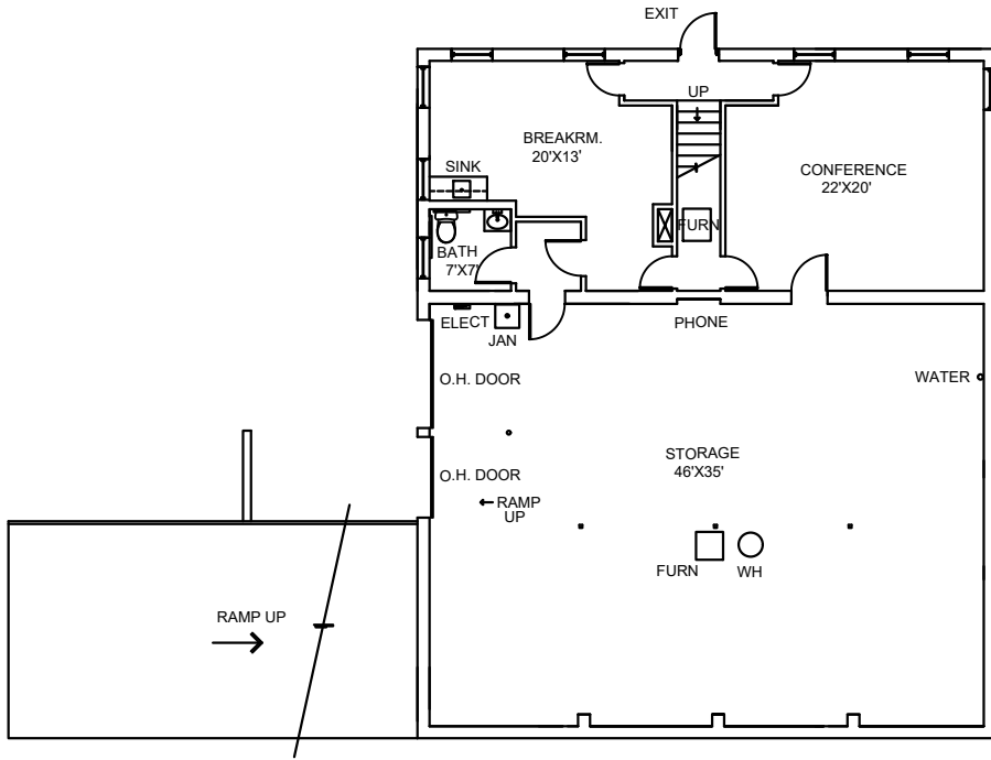
1203 FAY ST. LOWER LEVEL PLAN SCALE: 3/16"=1'-0" ON 24X36 PAPER 1,022 OFFICE + 1,740 GARAGE = 2,762 SF
