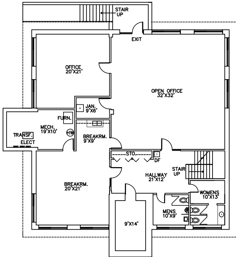
LOWER LEVEL 3,296 SF 2101 W. BROADWAY 3/16"=1'-0" SCALE ON 24 X 36 PAPER SM 9.23.25
