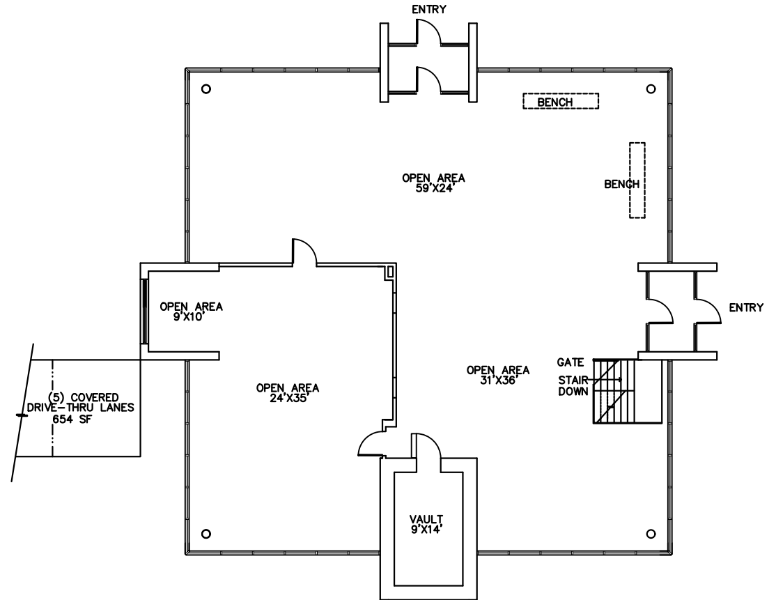
FIRST FLOOR PLAN 3,865 SF (NIC DRIVE-THRU LANES) 2101 W. BROADWAY 3/16"=1'-0" SCALE ON 24 X 36 PAPER SM 9.23.25
