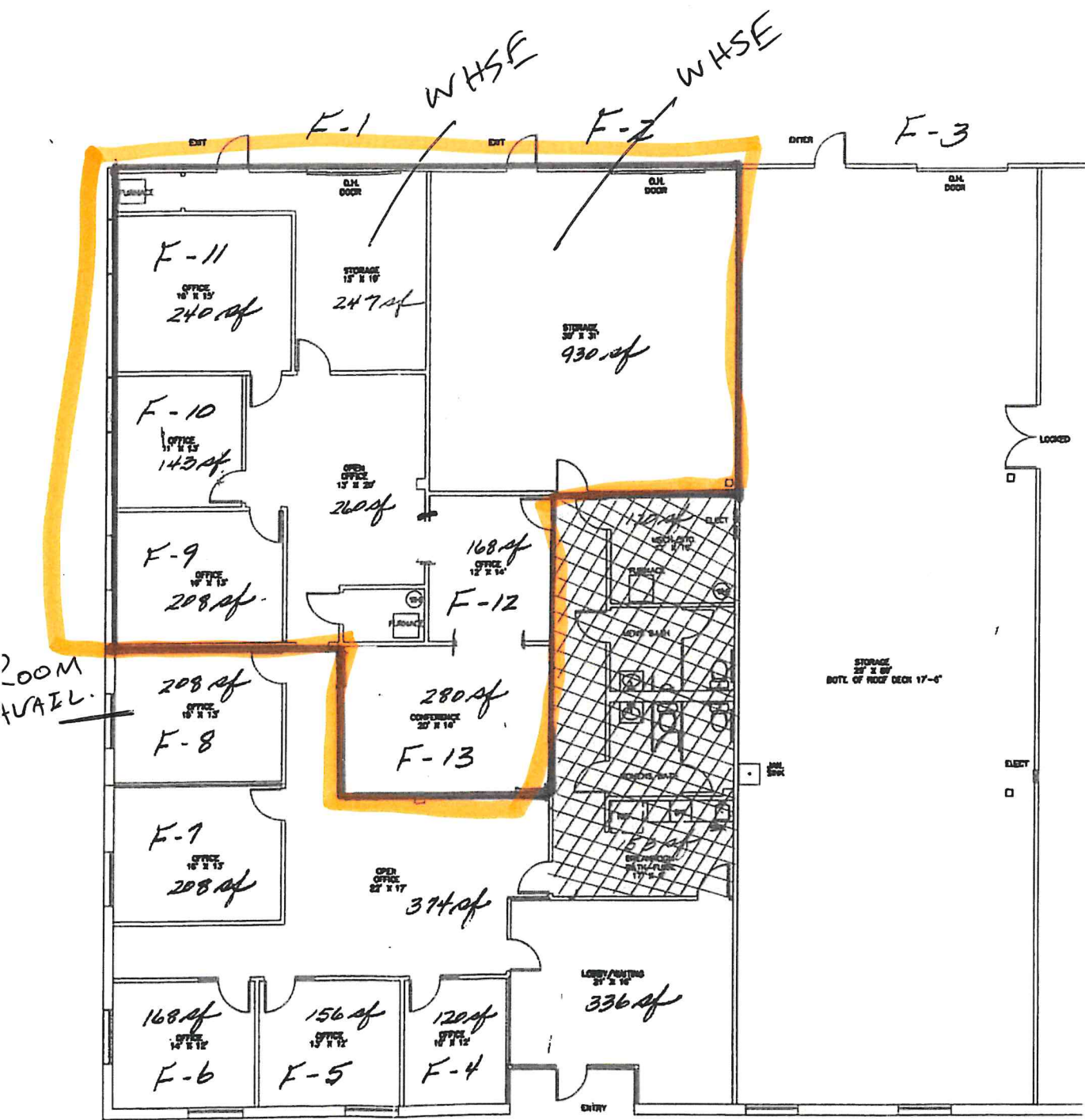
5800 N. TOWER DR. STE F FLOOR PLAN SCALE: 3/16" = 1'-0" 2-4-10 PRINT AT 24" x 36" PAPER
