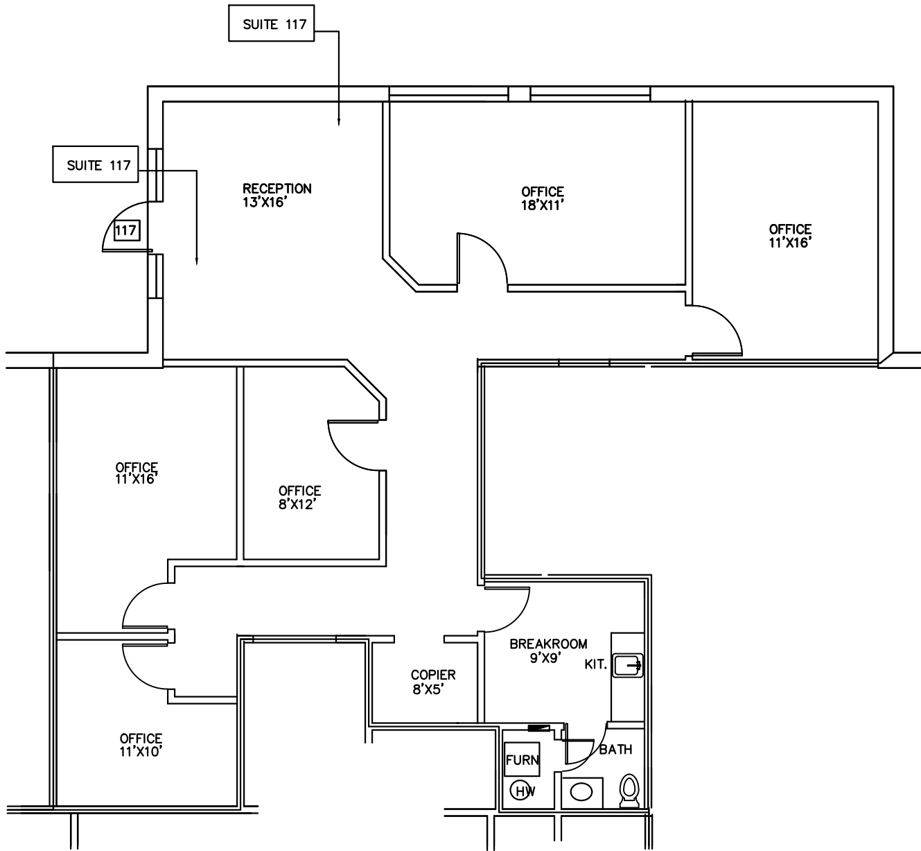
1ST FLOOR – FLOOR PLAN SCALE 1/8" = 1'-0" ON 8.5X11 PAPER
